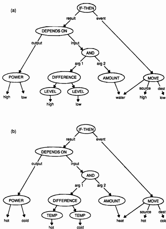
Figure 11.1. Carnot's analogy: the common relational structure for water and heat.
