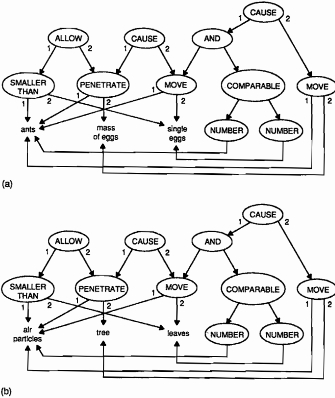
Figure 11.3. Boyle's analogy: the common relational structure for ants moving eggs and wind blowing leaves.
